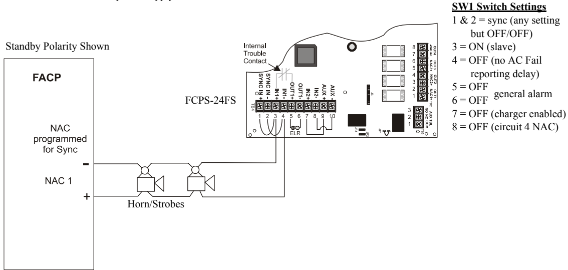
Figure 5.6 Supervised Master/Slave Connections
