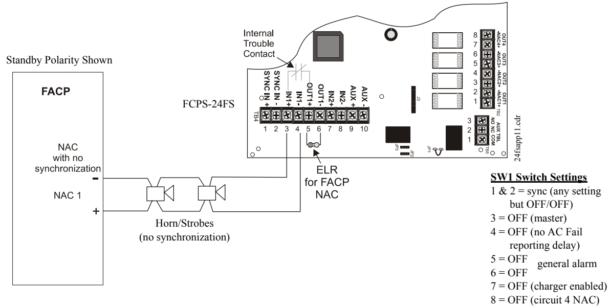
Figure 5.7 Supervised FACP to Master Connections (nonsynchronized source)
